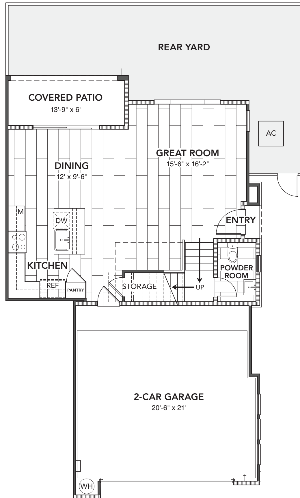
FIRST FLOOR
