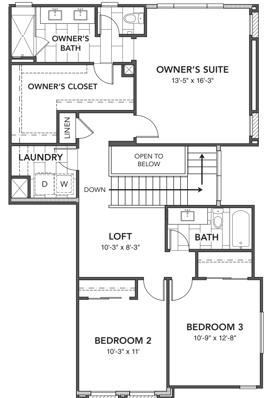
2ND FLOOR
